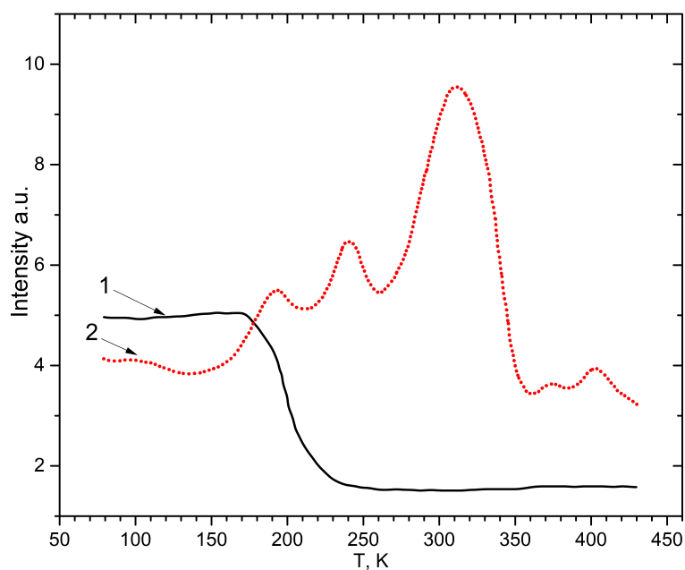
Figure 11. Temperature dependence of the main emissions arising from X-ray luminescence in \text{K}_2\text{SO}_4 - \text{Pb} .
